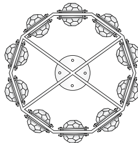
48" Diameter - 10 lights
