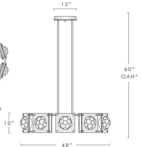
48" Diameter - 10 lights
